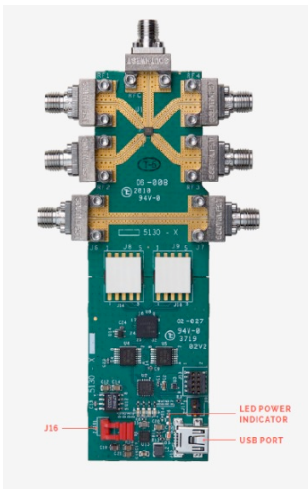
Figure 3:MM5130EVK2 18 GHz Evaluation Board
