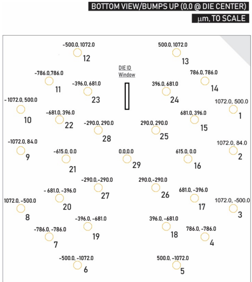
Figure 2: Bump Coordinates
